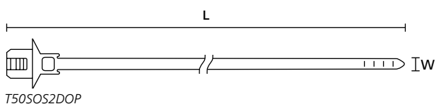
DOP versions for oval holes features anti-twist protection
