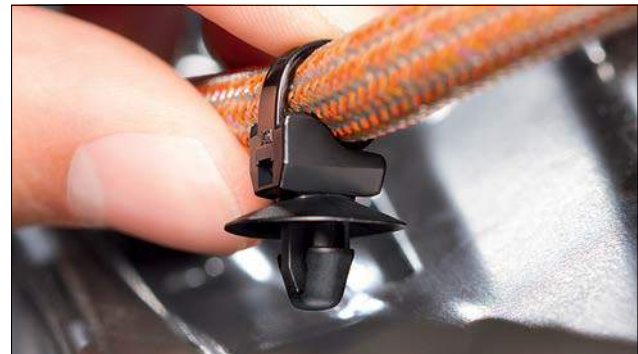
The Disc at the head of the T50SOSST6.5E protects the bore against dirt and splashes
