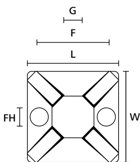
MCMB Mount
