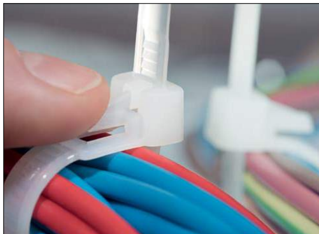
REL series can be opened with one hand
